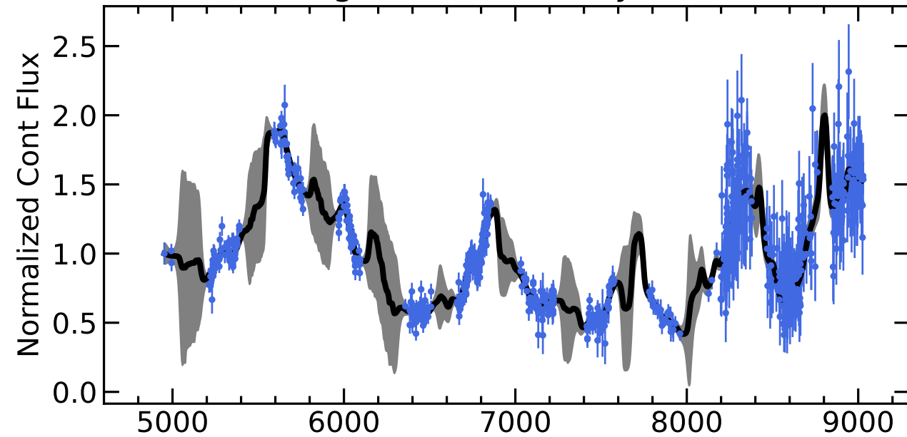
RM601 Light Curves (w/ PyROA model)
