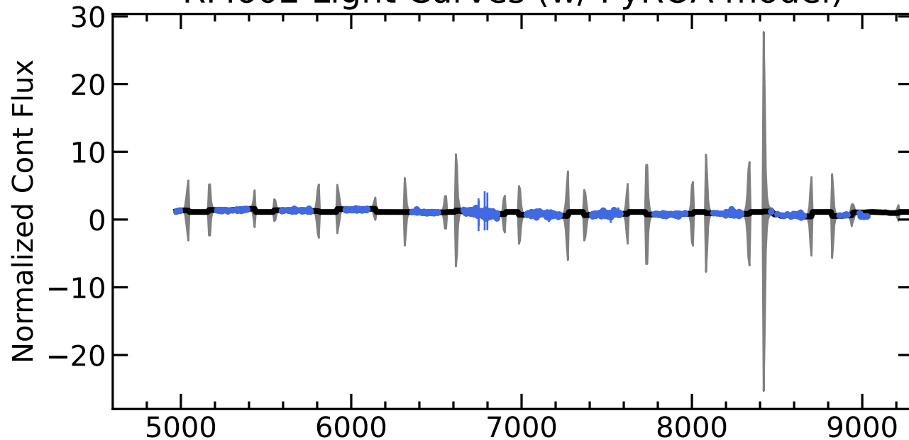
RM602 Light Curves (w/ PyROA model)
