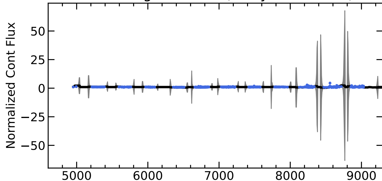
RM604 Light Curves (w/ PyROA model)
