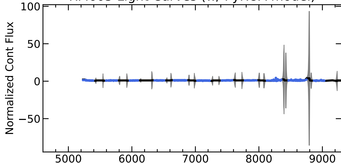
RM605 Light Curves (w/ PyROA model)
