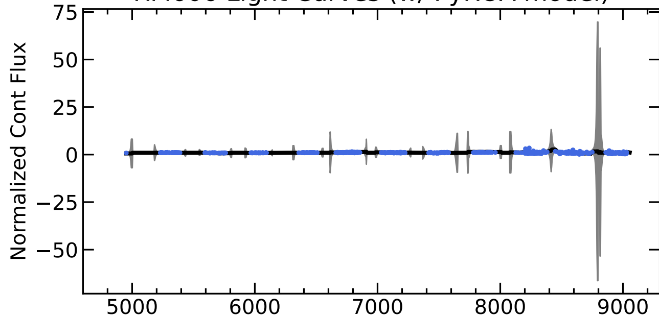
RM606 Light Curves (w/ PyROA model)
