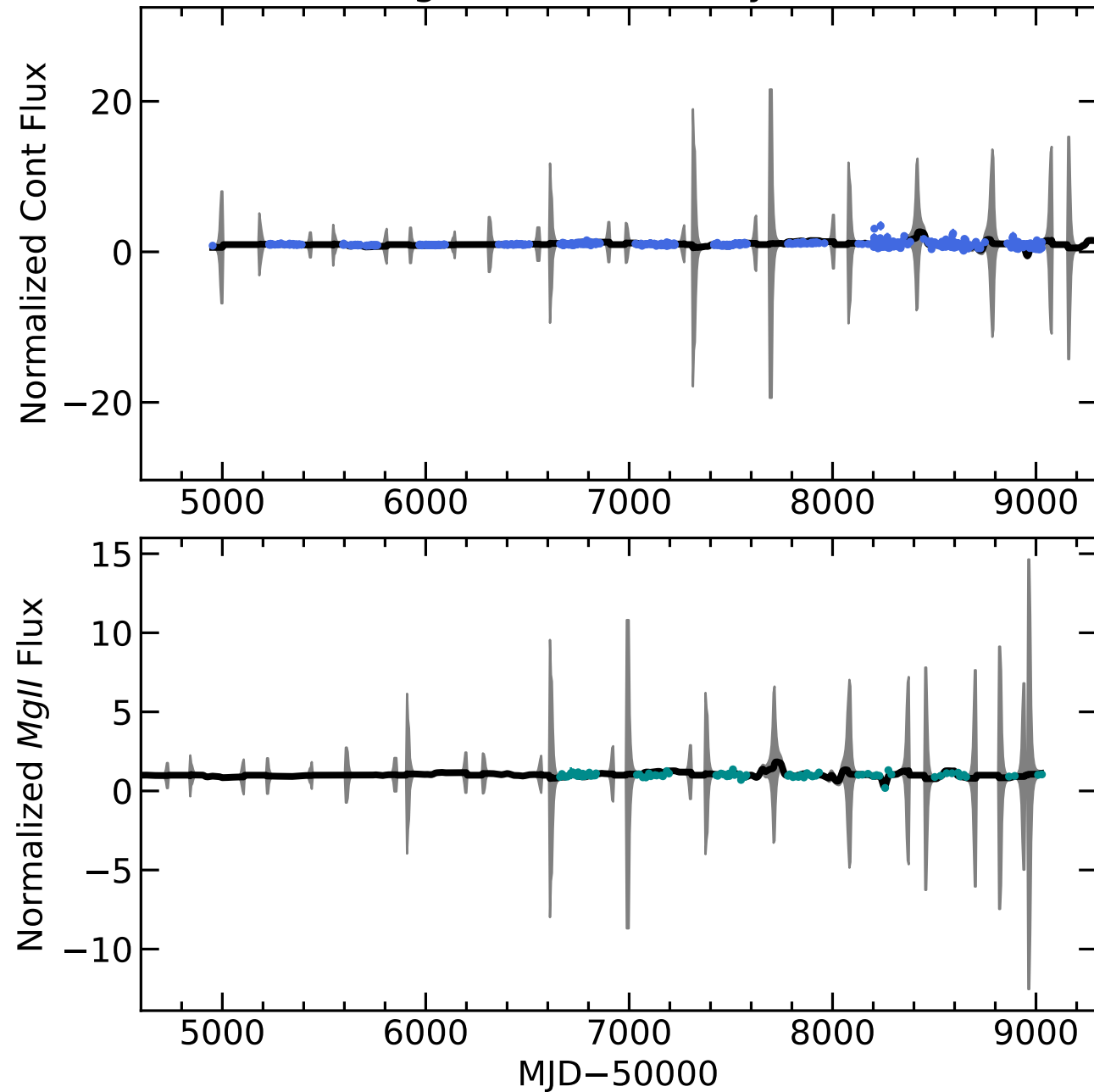
RM606 Light Curves (w/ PyROA model)
