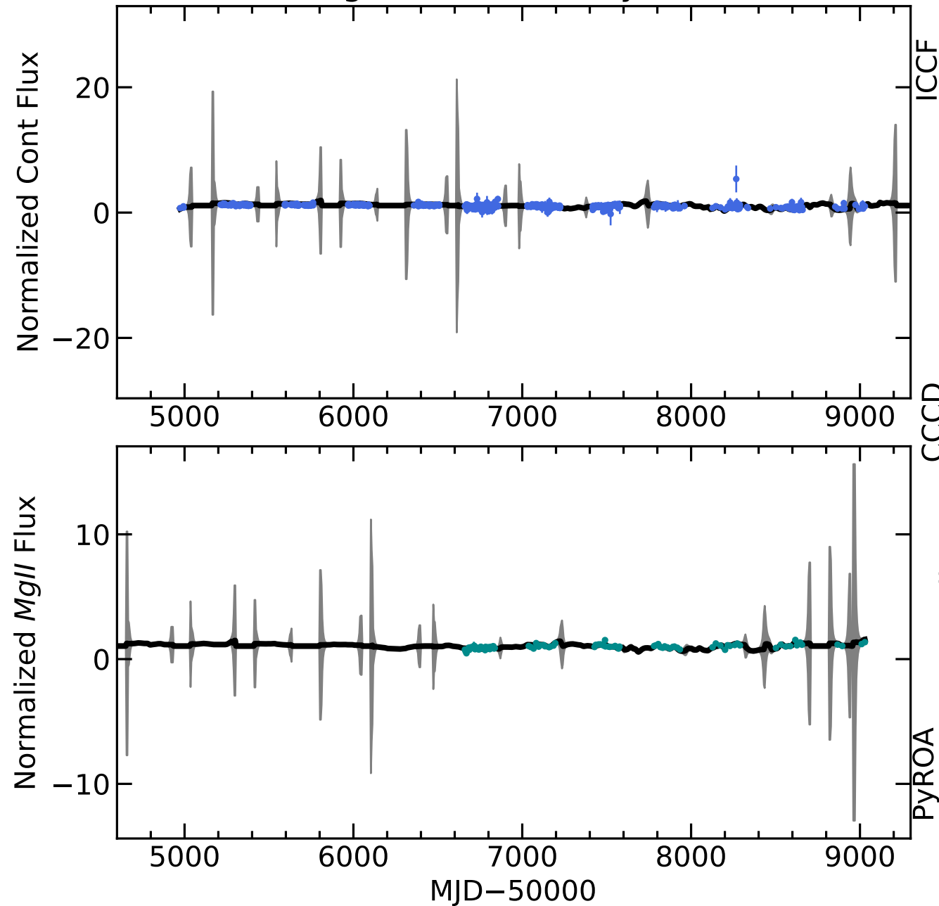
RM607 Light Curves (w/ PyROA model)
