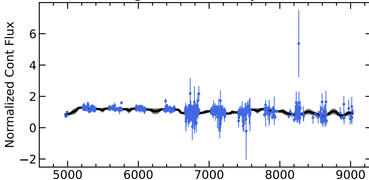
RM607 Light Curves (w/ PyROA model)
