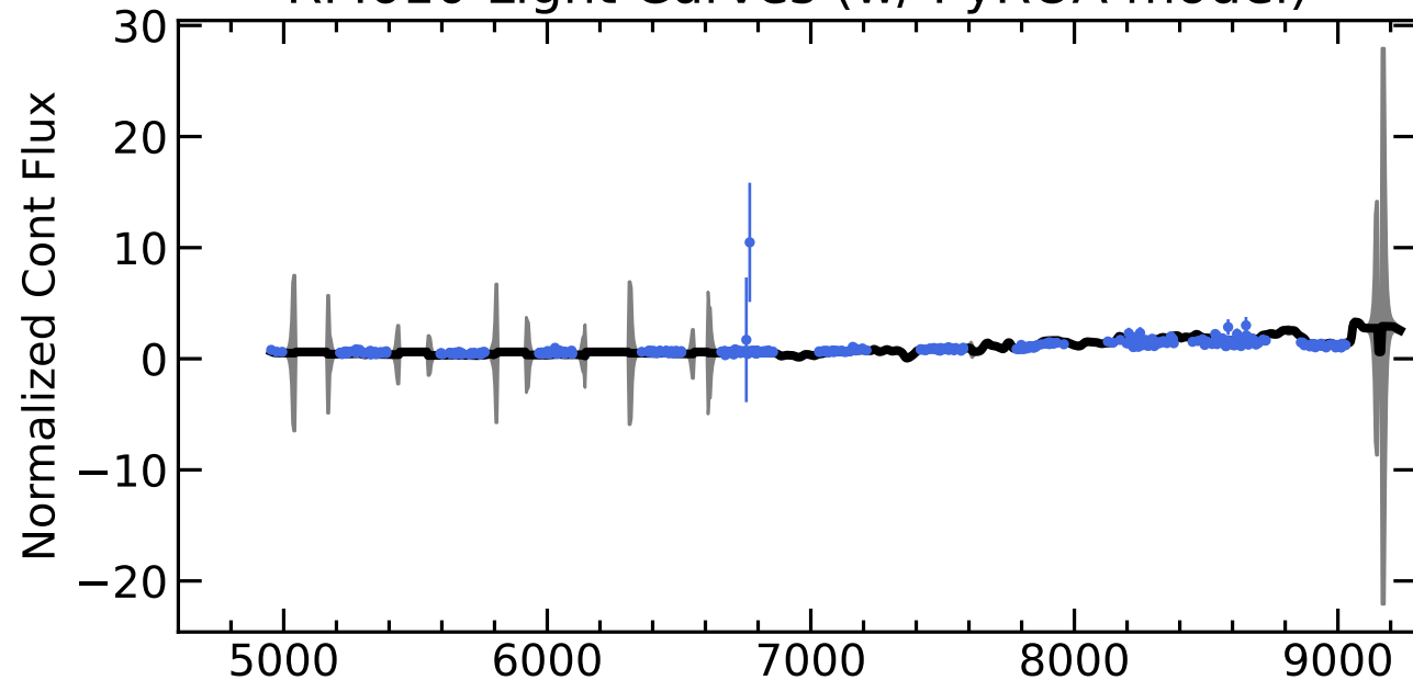
RM610 Light Curves (w/ PyROA model)
