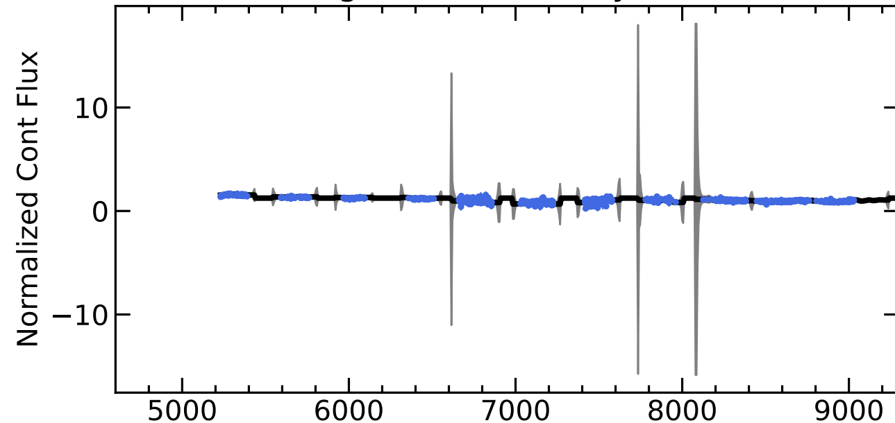
RM611 Light Curves (w/ PyROA model)
