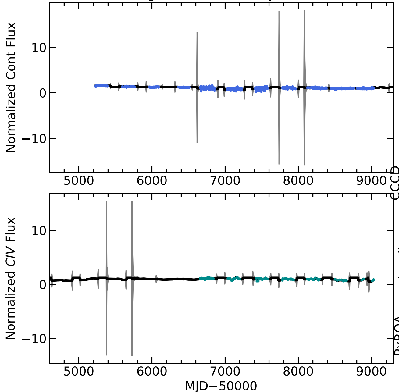
RM611 Light Curves (w/ PyROA model)
