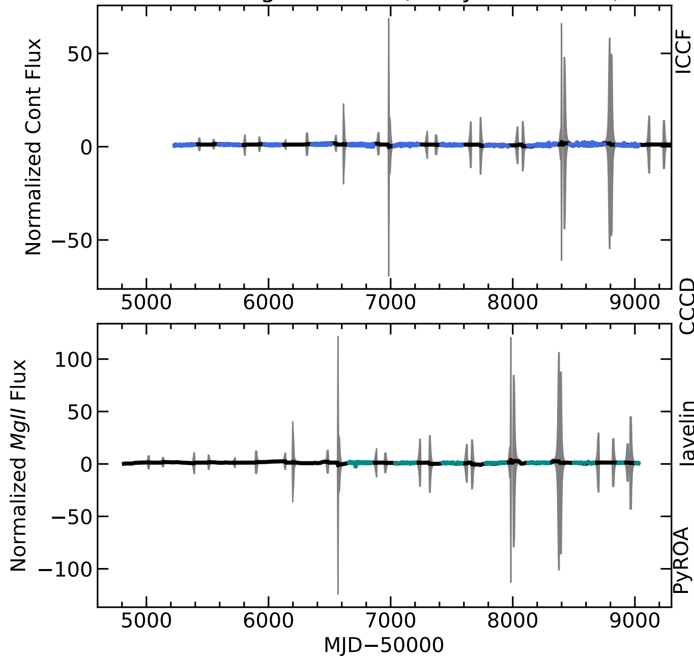
RM612 Light Curves (w/ PyROA model)
