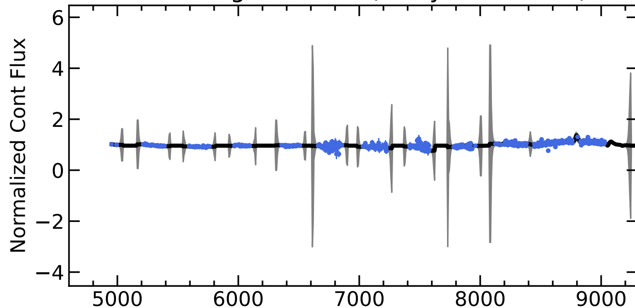
RM613 Light Curves (w/ PyROA model)
