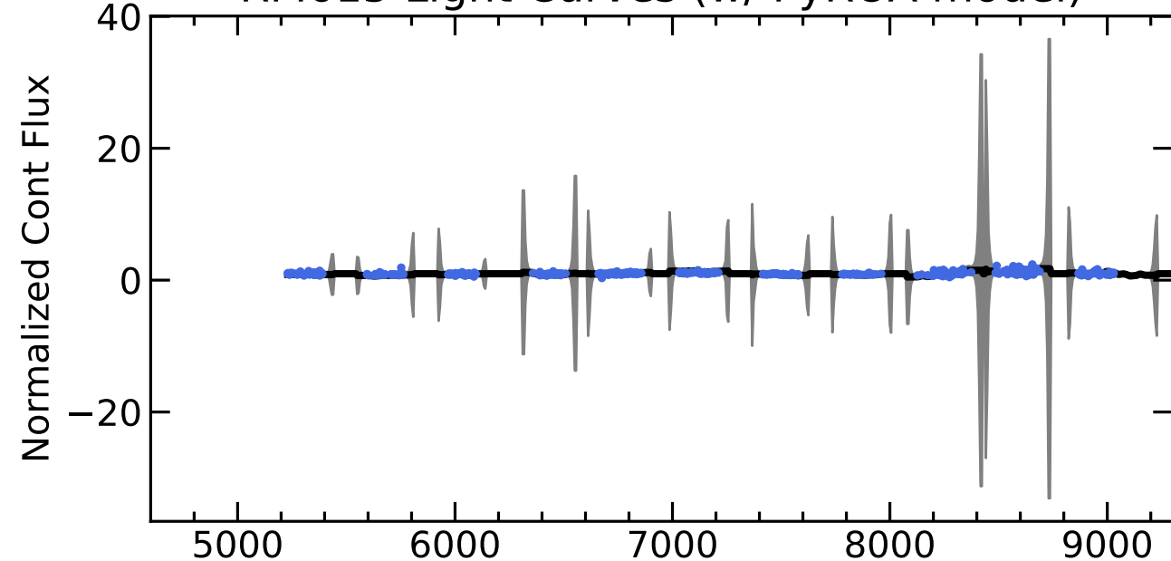
RM615 Light Curves (w/ PyROA model)
