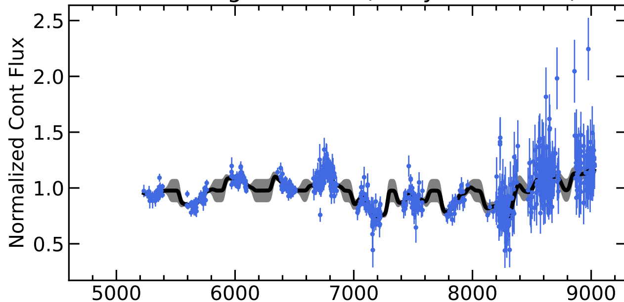
RM617 Light Curves (w/ PyROA model)
