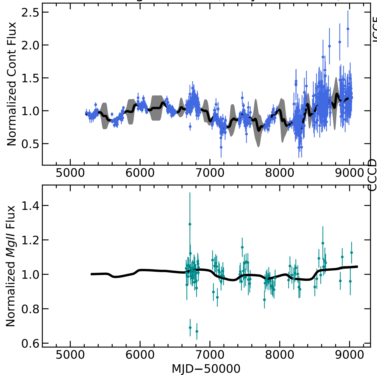
RM617 Light Curves (w/ PyROA model)
