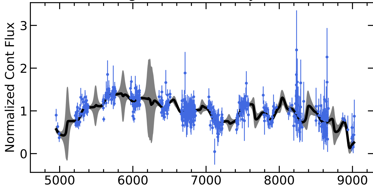
RM618 Light Curves (w/ PyROA model)
