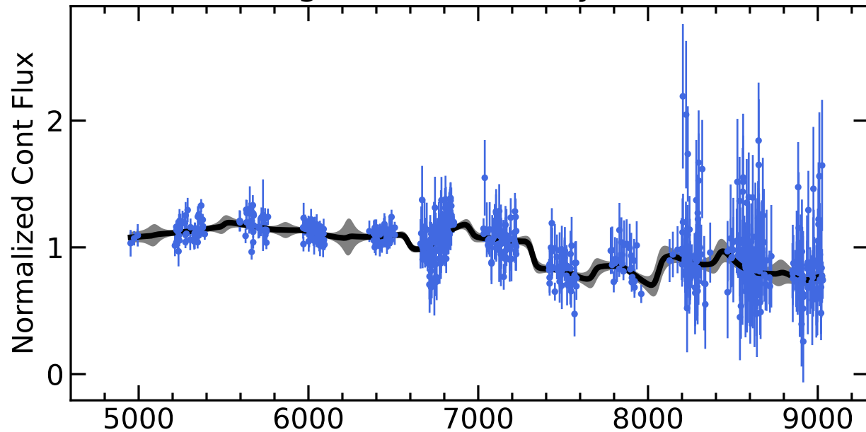
RM619 Light Curves (w/ PyROA model)
