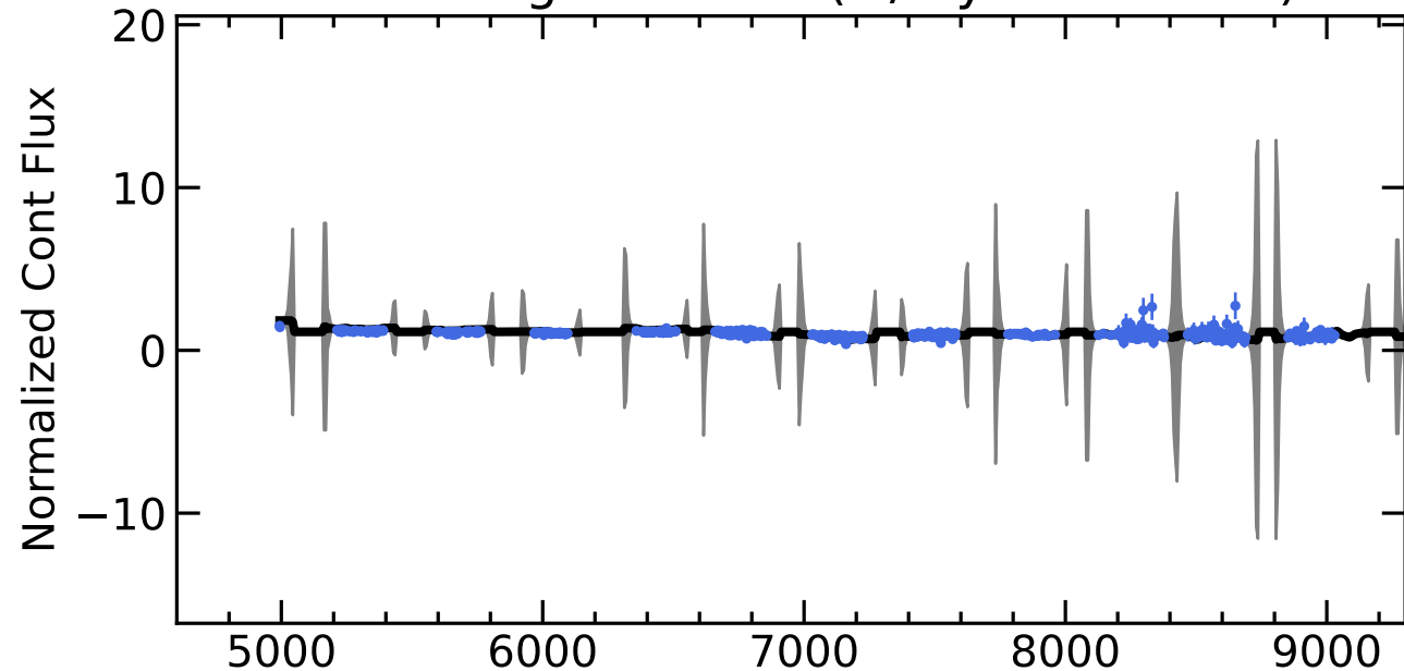
RM620 Light Curves (w/ PyROA model)
