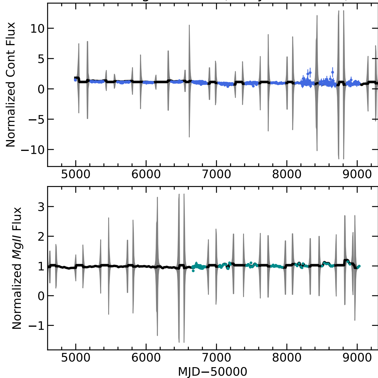
RM620 Light Curves (w/ PyROA model)
