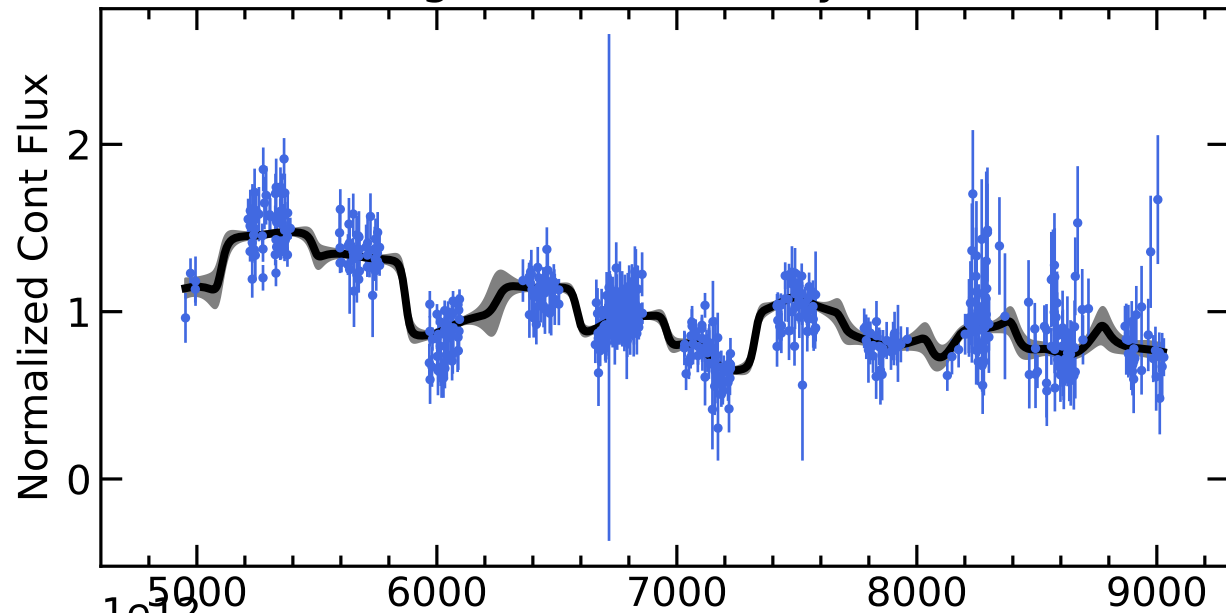
RM621 Light Curves (w/ PyROA model)
