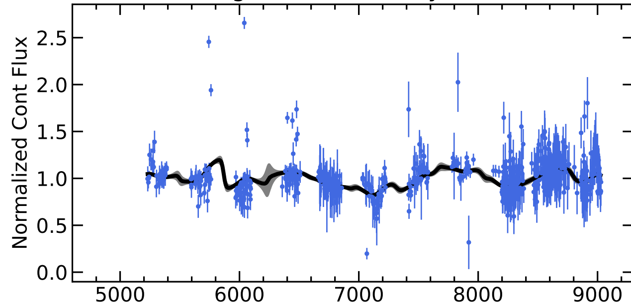
RM622 Light Curves (w/ PyROA model)
