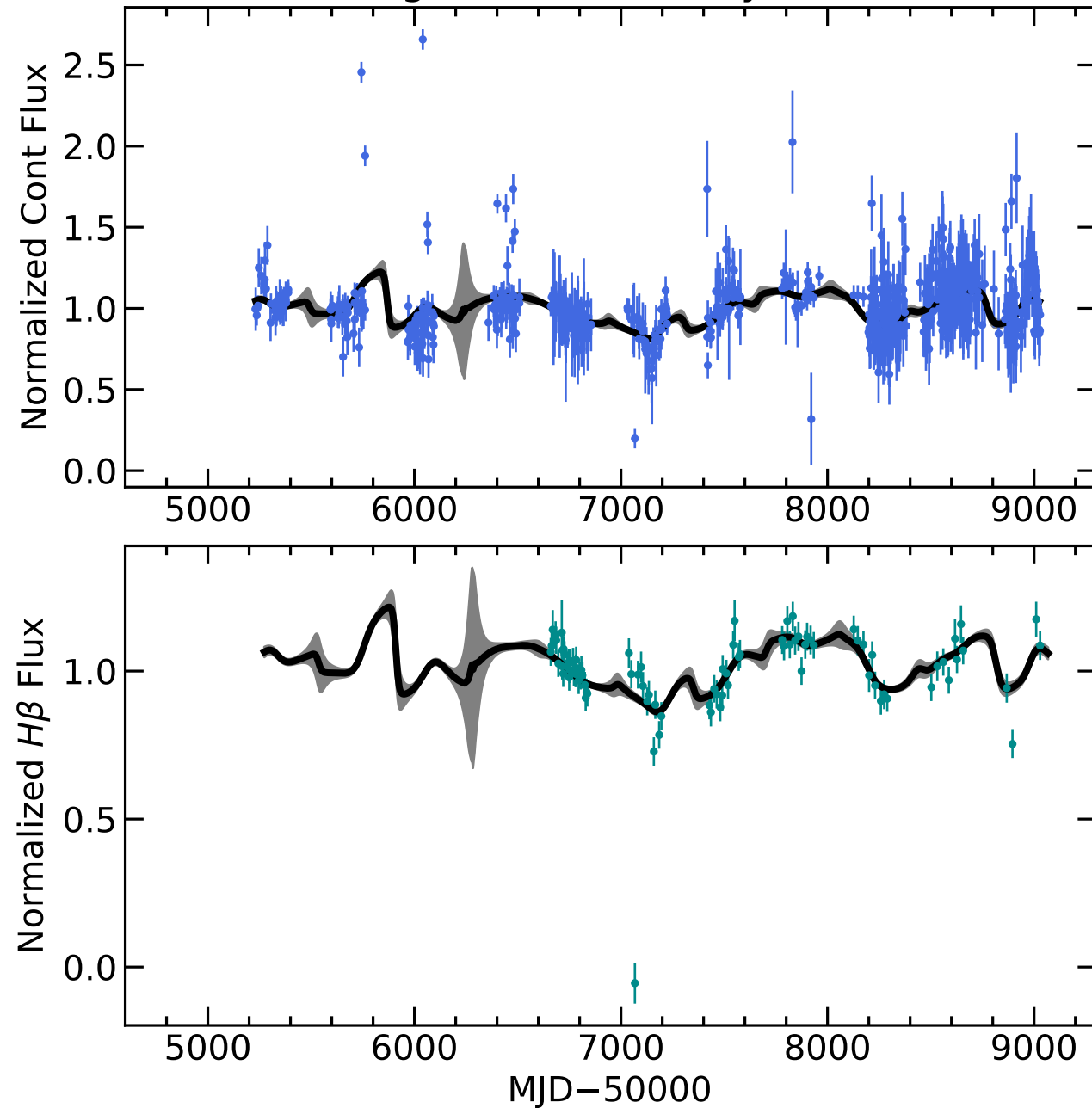
RM622 Light Curves (w/ PyROA model)
