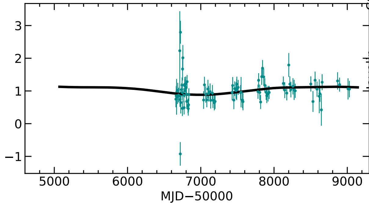
Normalized MgII Flux
