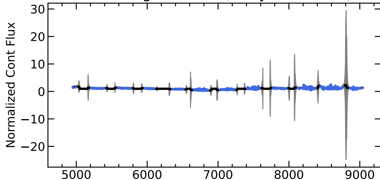
RM624 Light Curves (w/ PyROA model)
