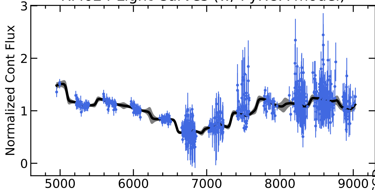
RM624 Light Curves (w/ PyROA model)
