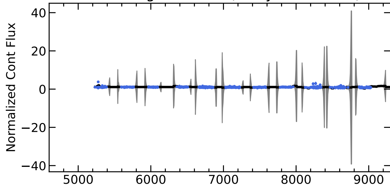
RM625 Light Curves (w/ PyROA model)
