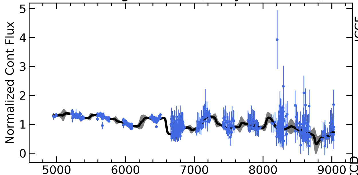
RM626 Light Curves (w/ PyROA model)
