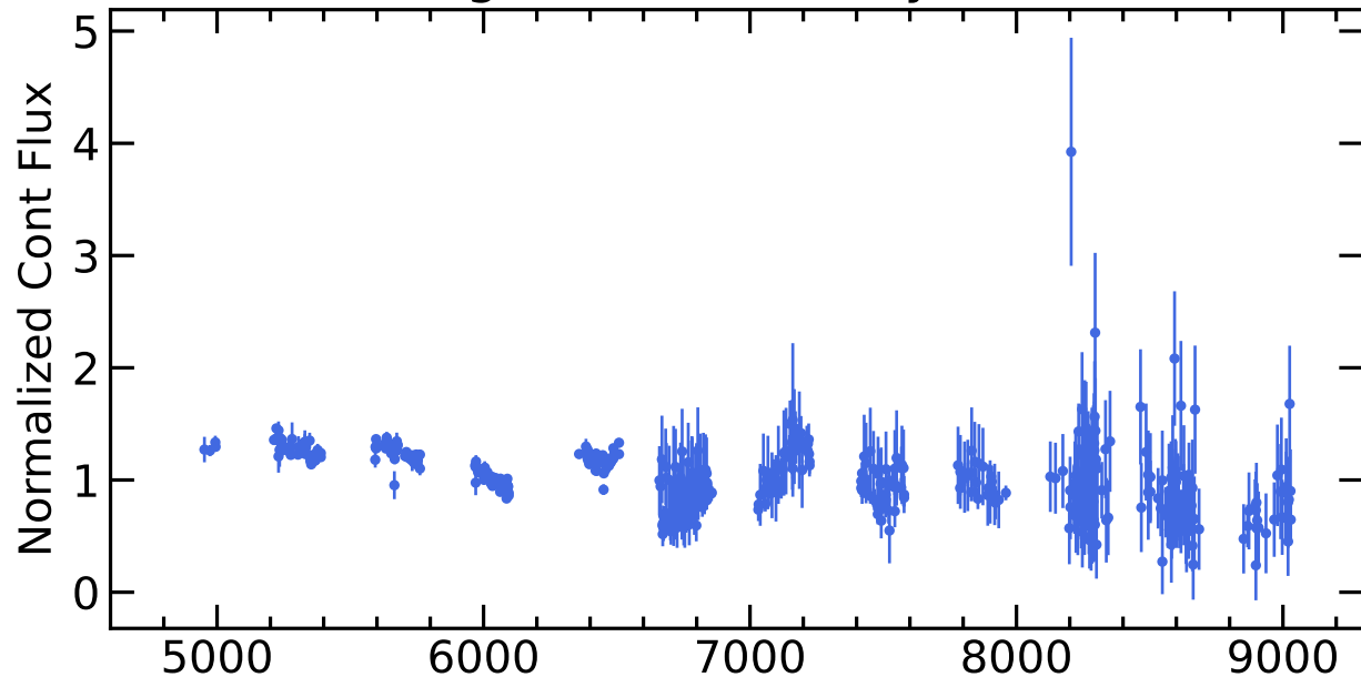
RM626 Light Curves (w/ PyROA model)
