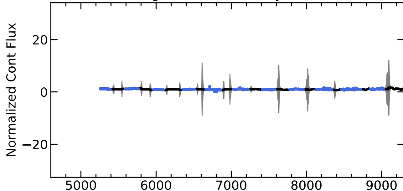
RM627 Light Curves (w/ PyROA model)
