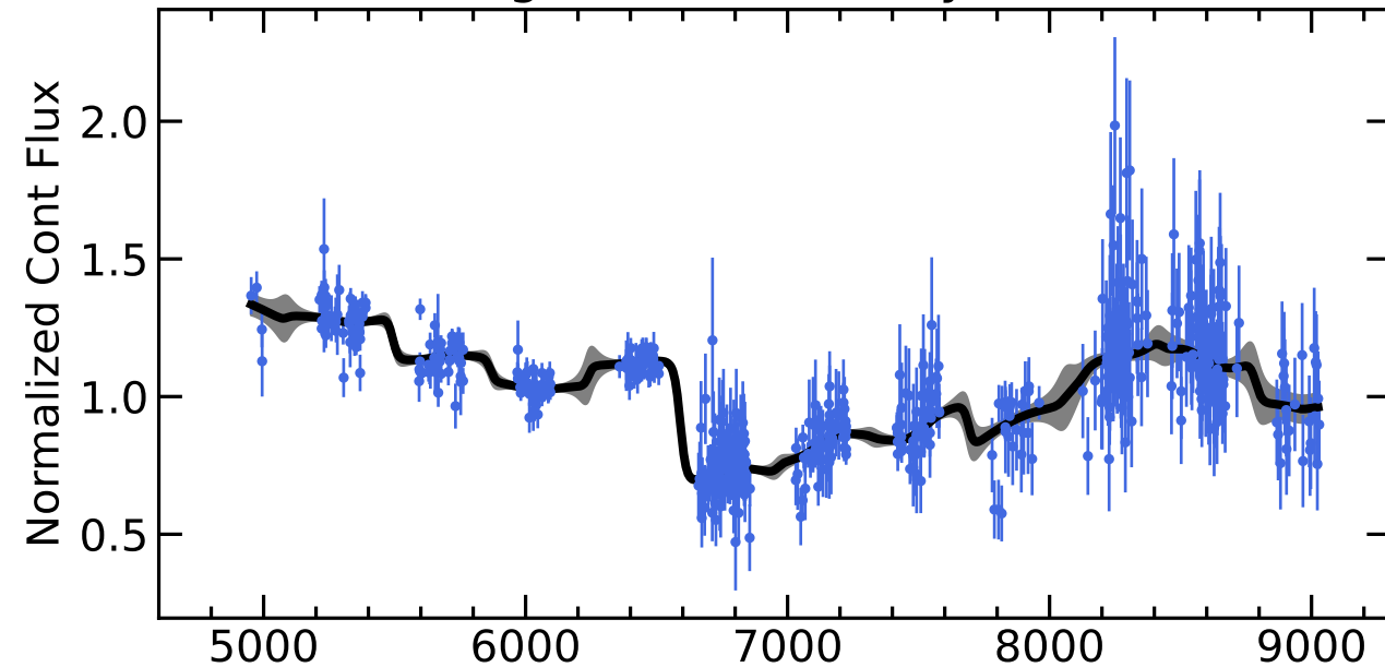
RM628 Light Curves (w/ PyROA model)
