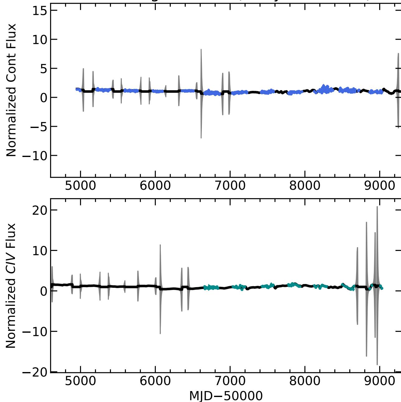
RM628 Light Curves (w/ PyROA model)
