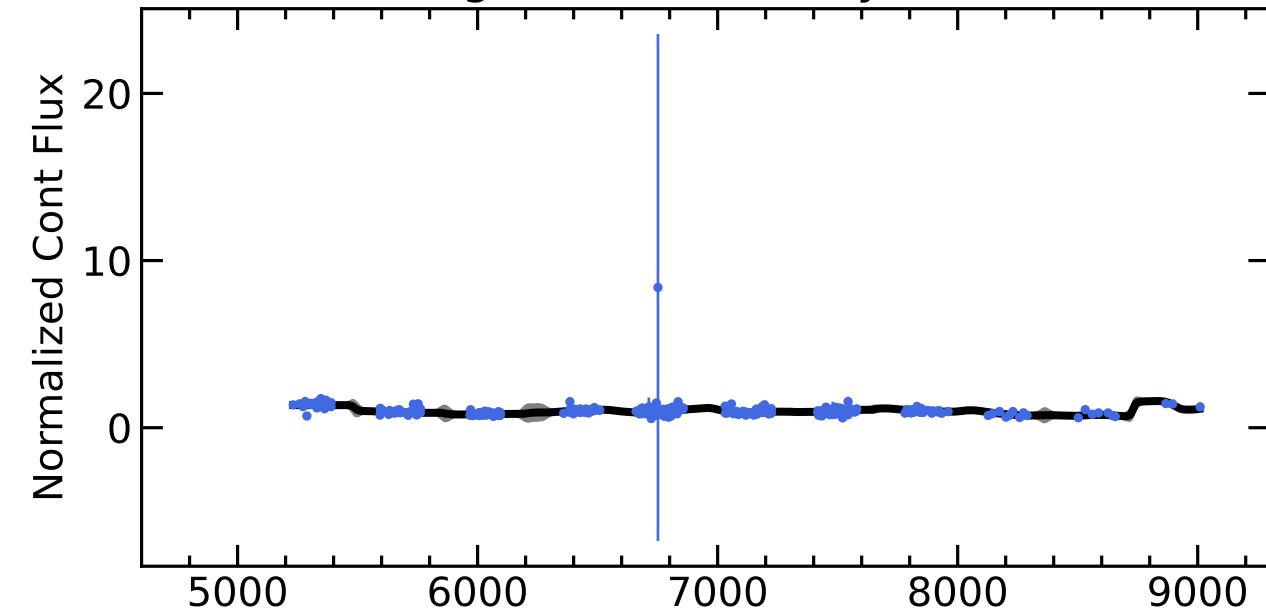
RM629 Light Curves (w/ PyROA model)
