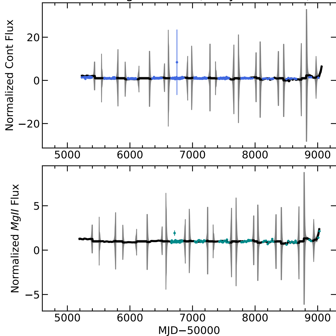
RM629 Light Curves (w/ PyROA model)
