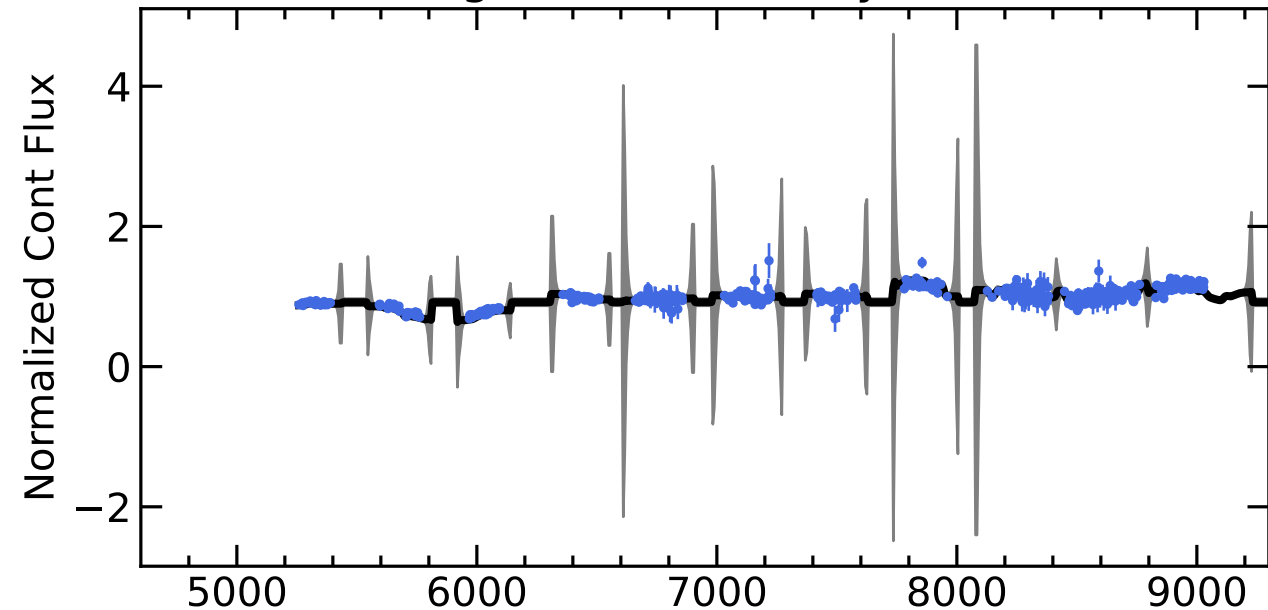
RM630 Light Curves (w/ PyROA model)
