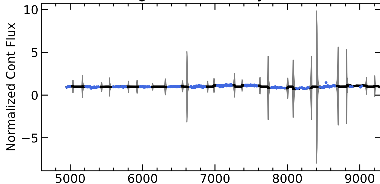
RM631 Light Curves (w/ PyROA model)
