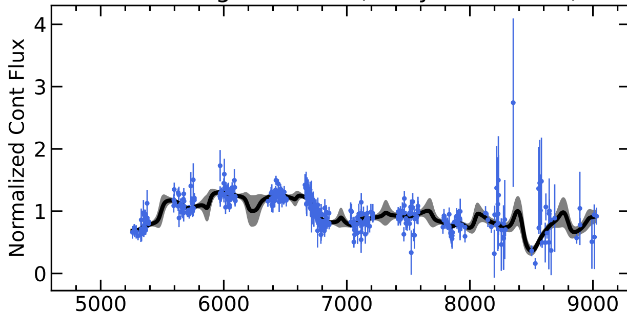
RM632 Light Curves (w/ PyROA model)
