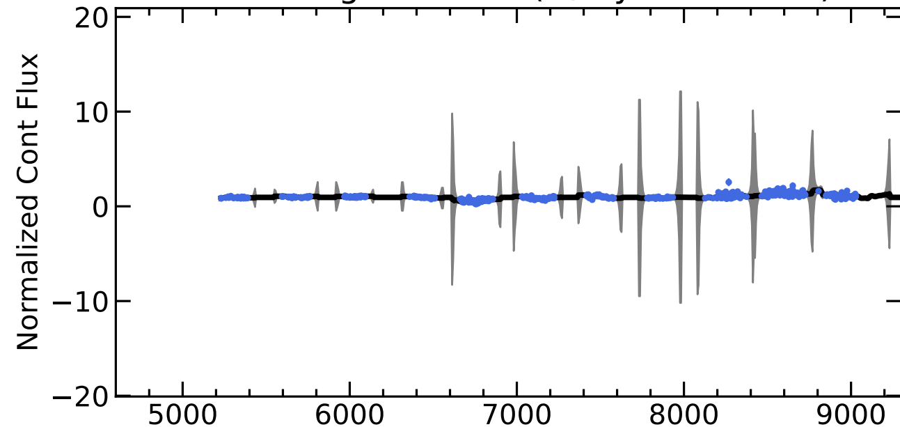
RM633 Light Curves (w/ PyROA model)
