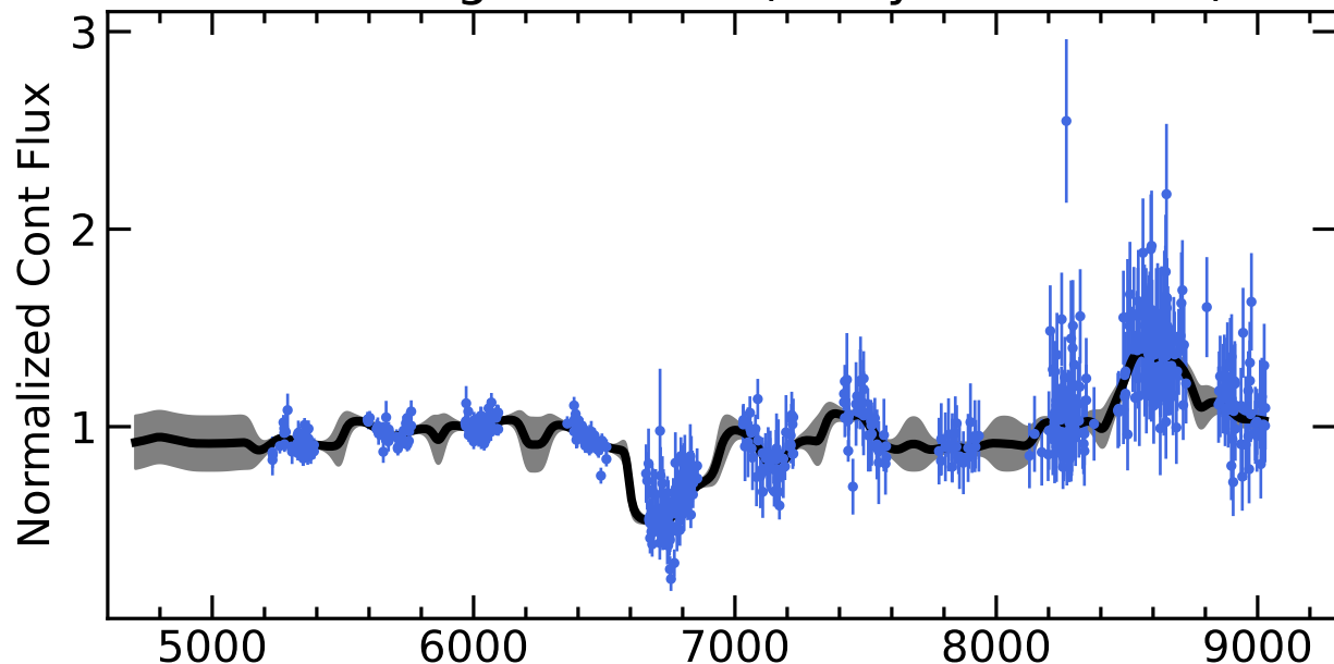
RM633 Light Curves (w/ PyROA model)
