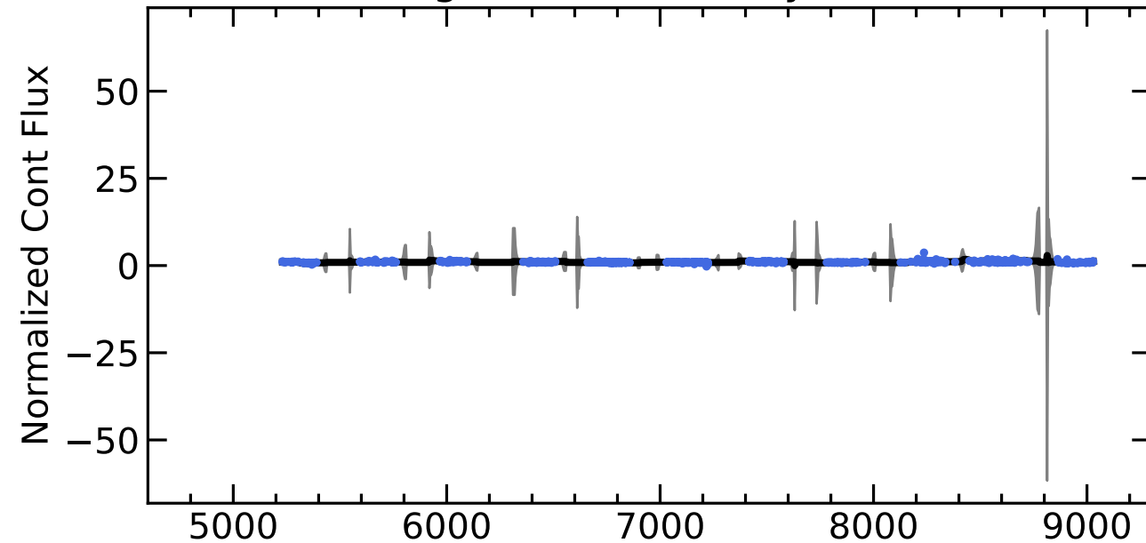
RM634 Light Curves (w/ PyROA model)
