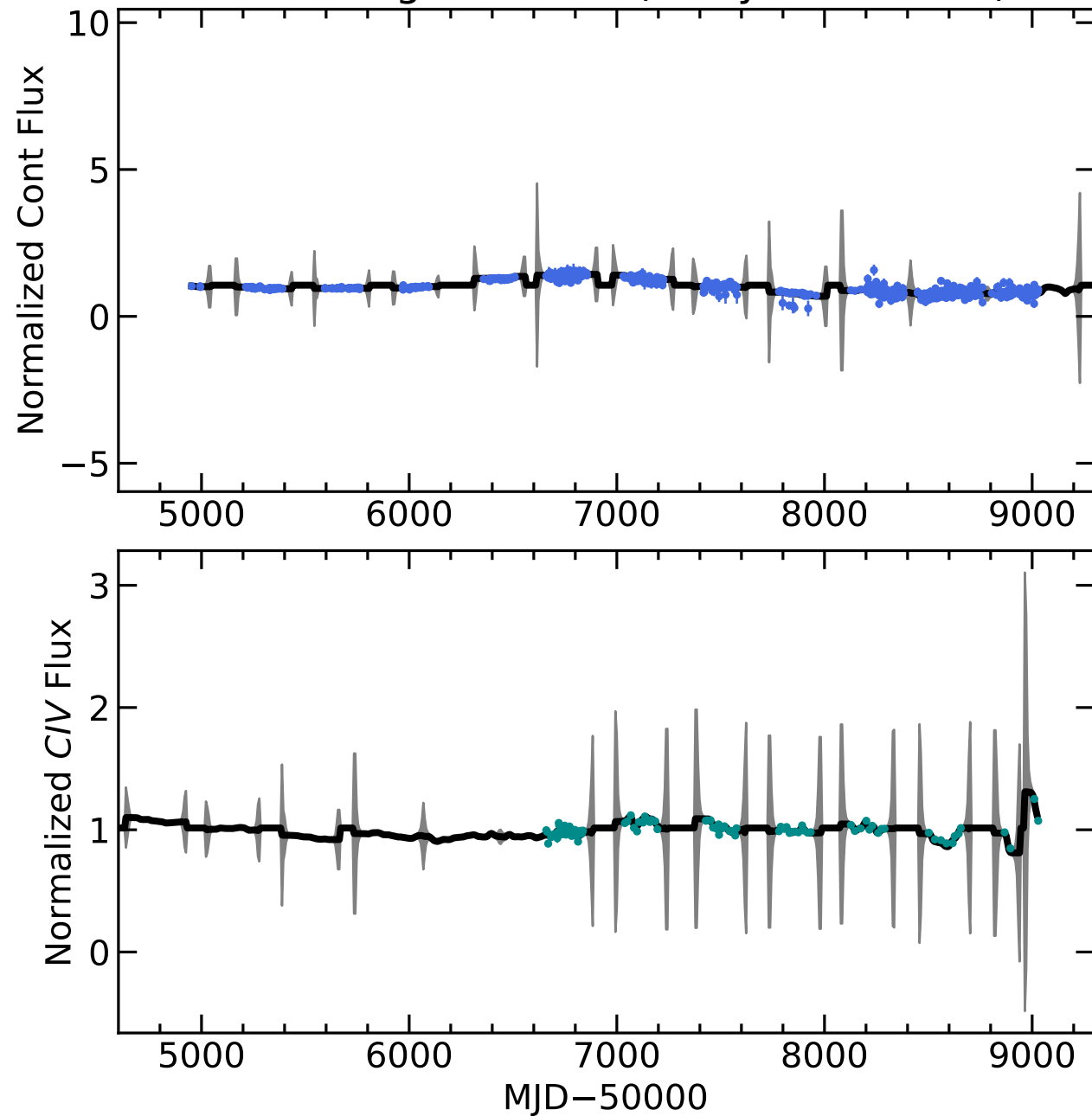
RM635 Light Curves (w/ PyROA model)
