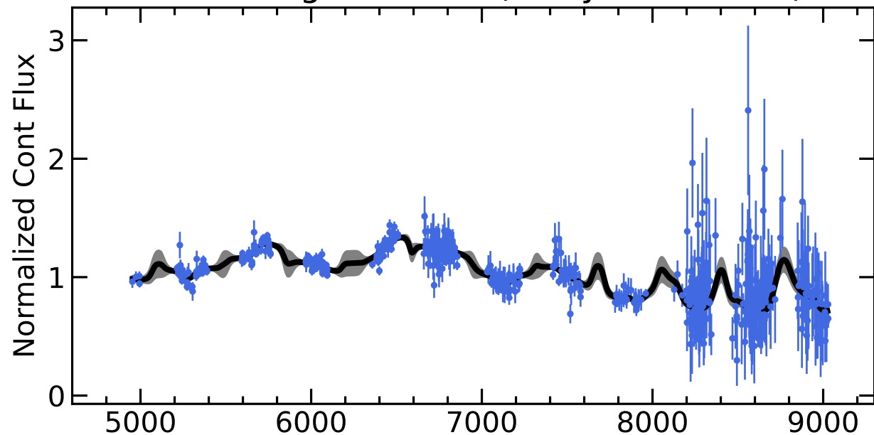
RM636 Light Curves (w/ PyROA model)
