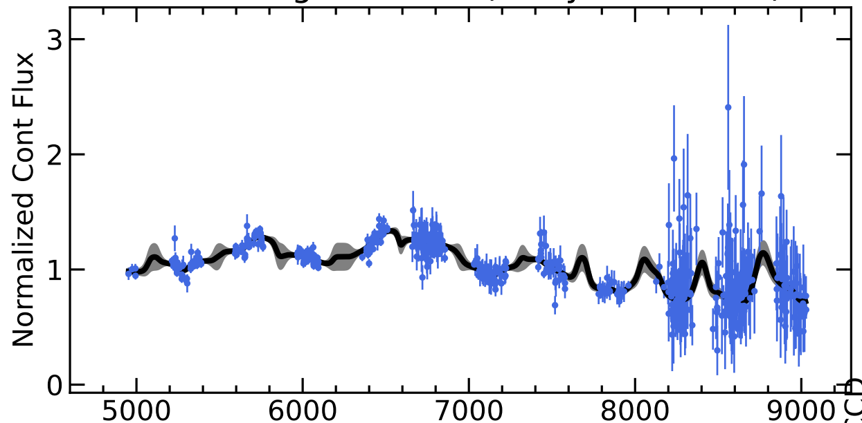
RM636 Light Curves (w/ PyROA model)
