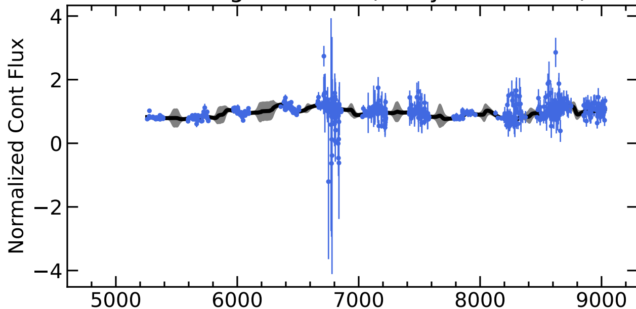
RM638 Light Curves (w/ PyROA model)
