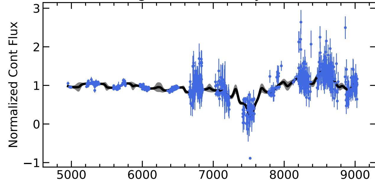
RM640 Light Curves (w/ PyROA model)
