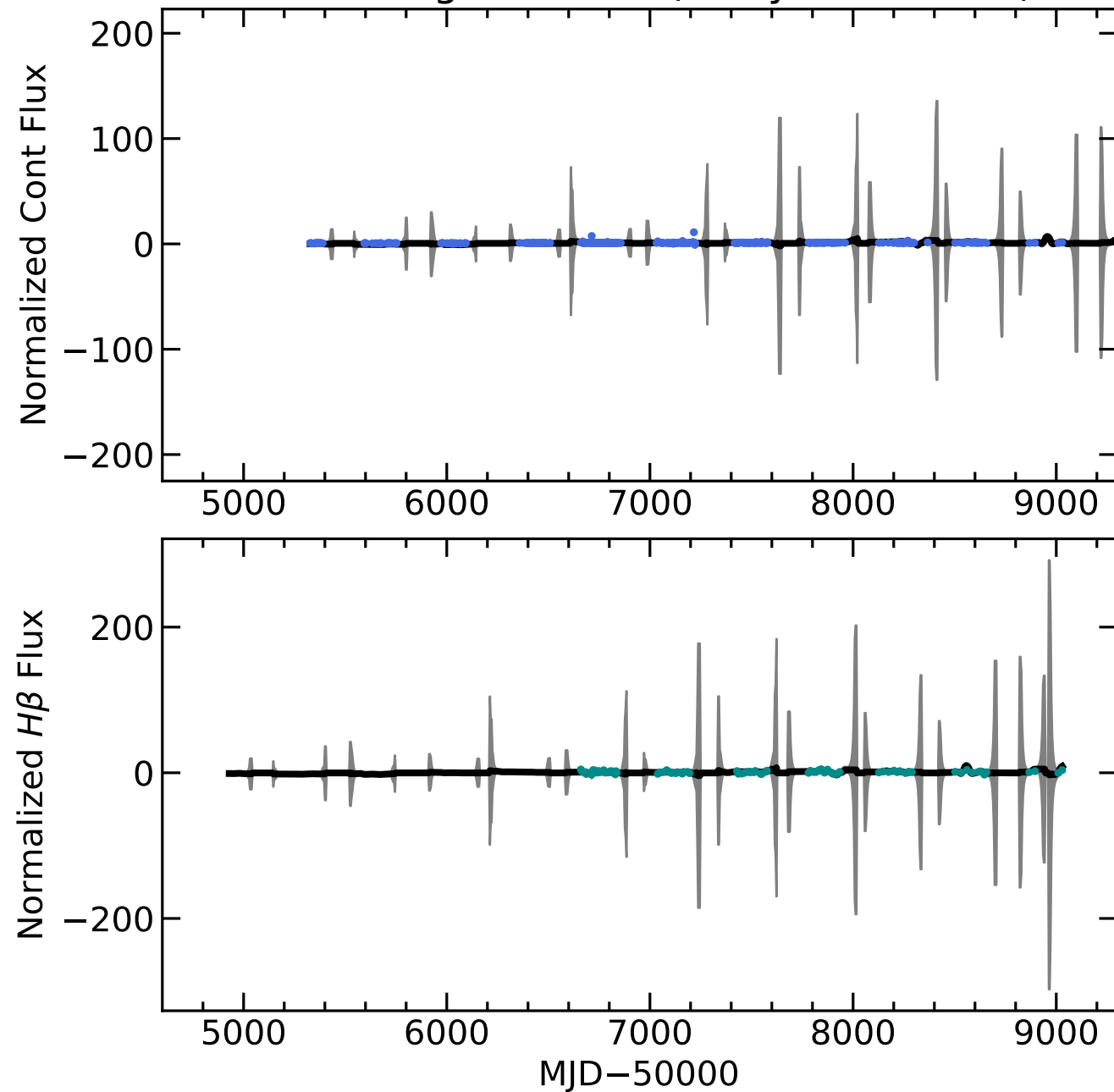
RM641 Light Curves (w/ PyROA model)
