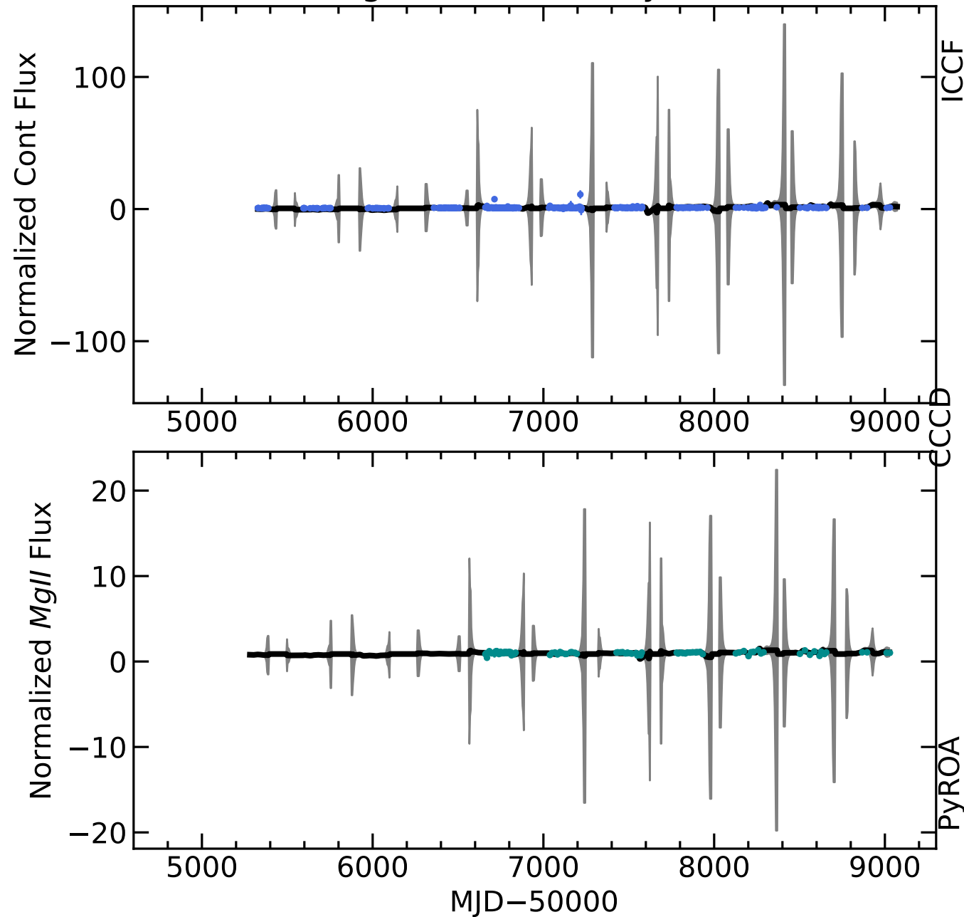
RM641 Light Curves (w/ PyROA model)
