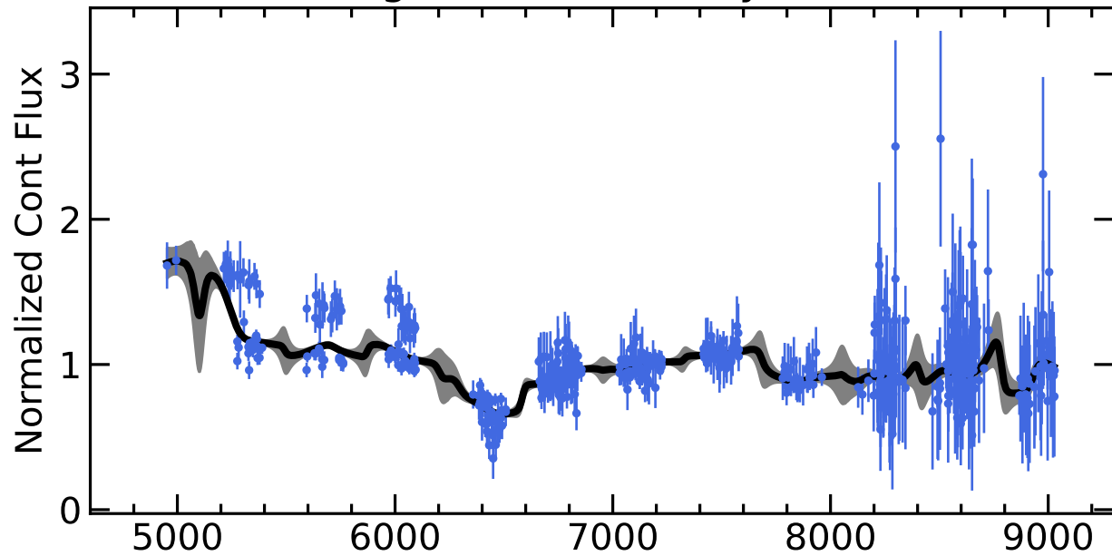
RM642 Light Curves (w/ PyROA model)
