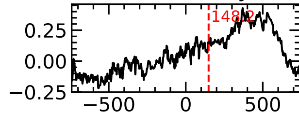
ICCF
