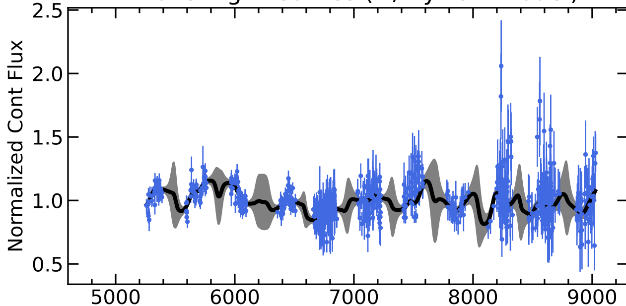
RM643 Light Curves (w/ PyROA model)
