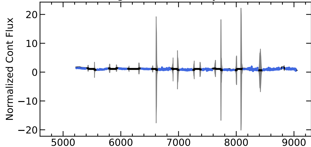
RM644 Light Curves (w/ PyROA model)
