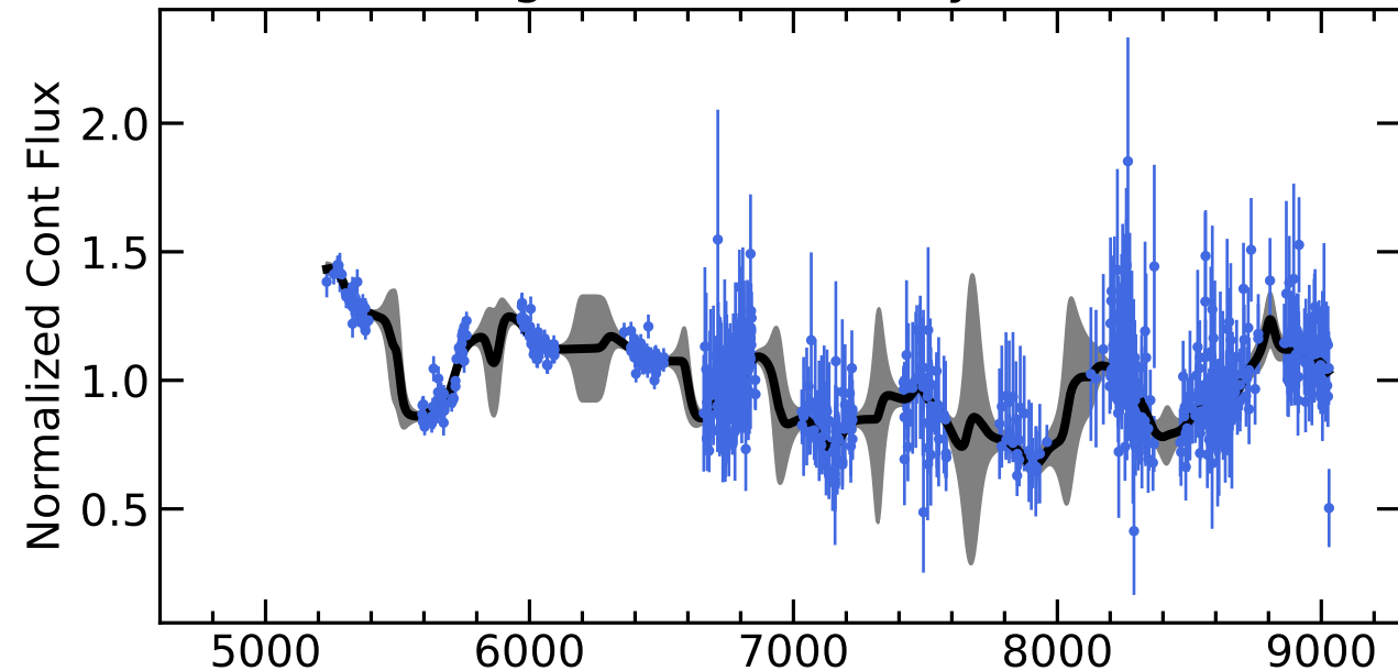
RM644 Light Curves (w/ PyROA model)
