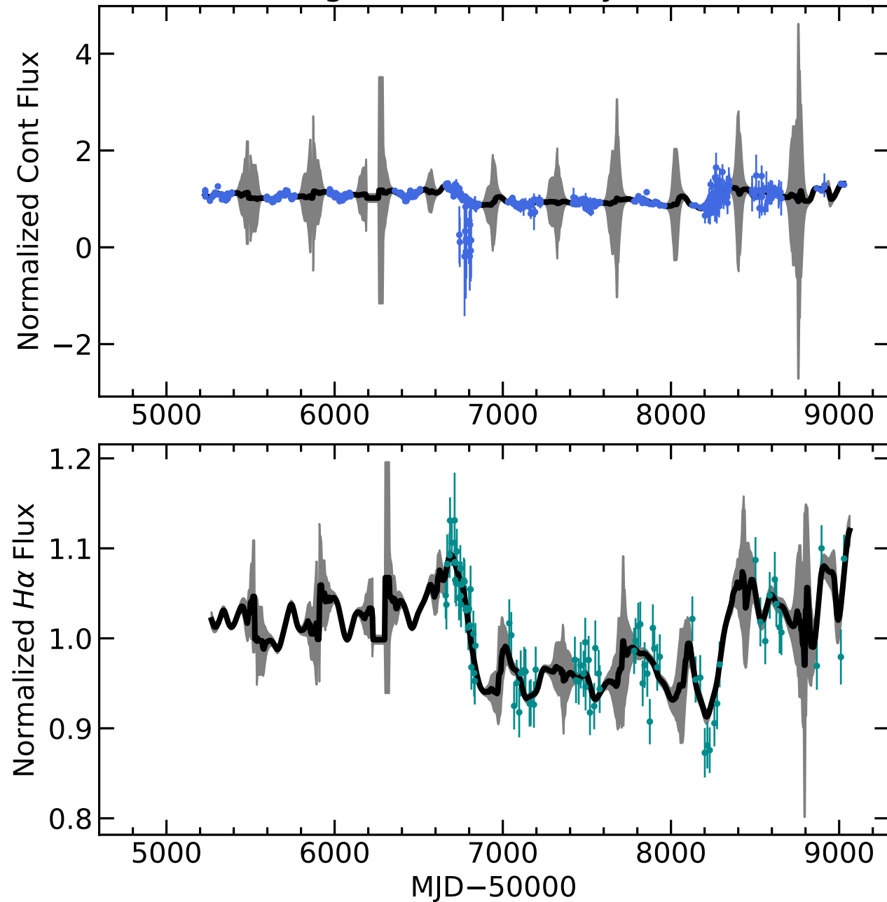
RM645 Light Curves (w/ PyROA model)
