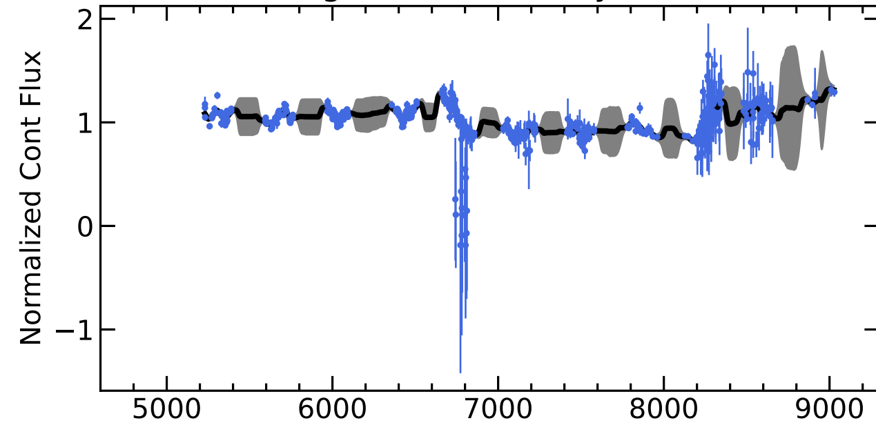
RM645 Light Curves (w/ PyROA model)
