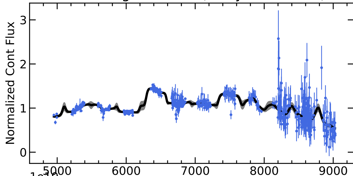
RM646 Light Curves (w/ PyROA model)
