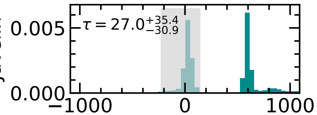
Javelin
