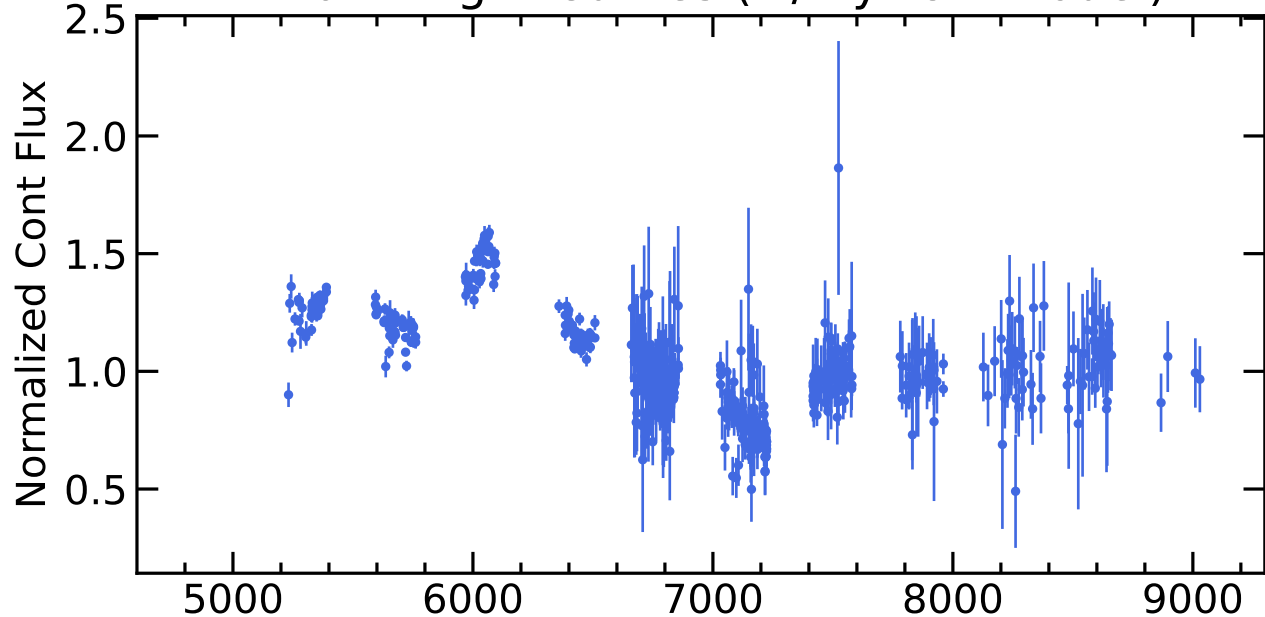
RM647 Light Curves (w/ PyROA model)
