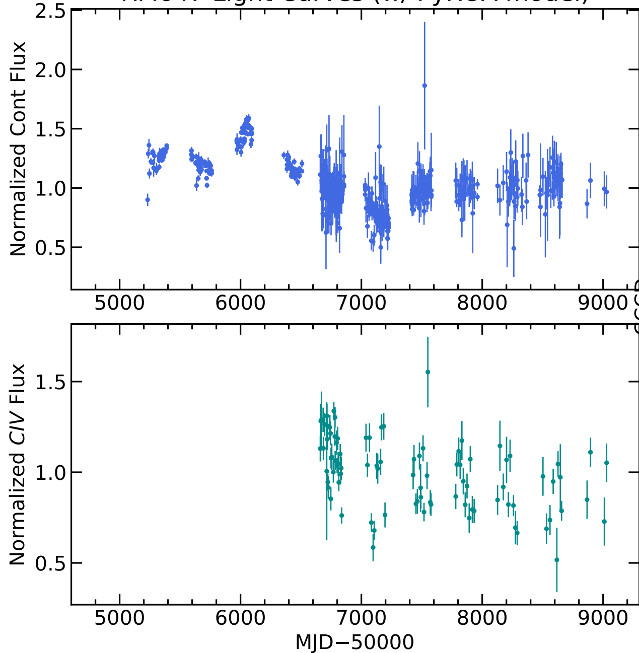
RM647 Light Curves (w/ PyROA model)
