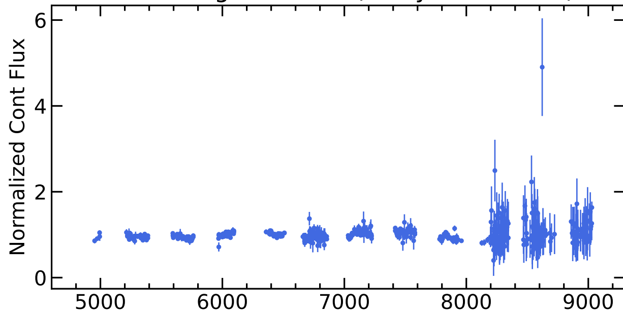
RM648 Light Curves (w/ PyROA model)
