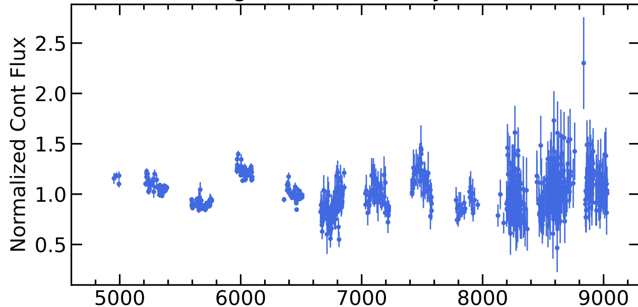
RM649 Light Curves (w/ PyROA model)
