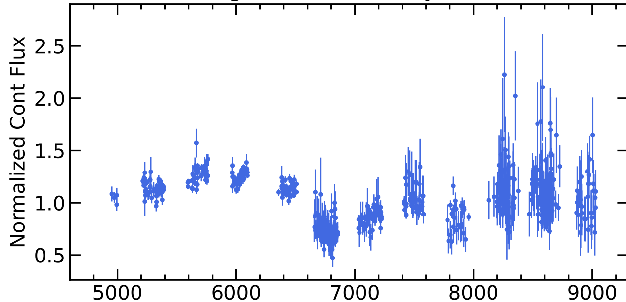
RM650 Light Curves (w/ PyROA model)
