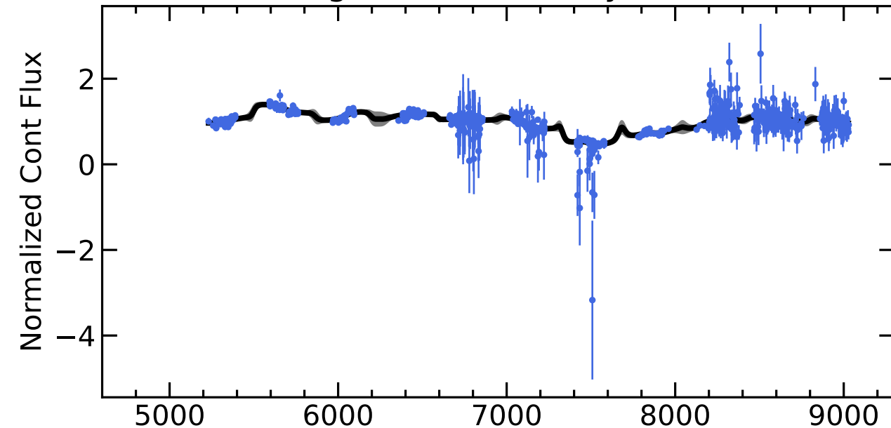
RM651 Light Curves (w/ PyROA model)
