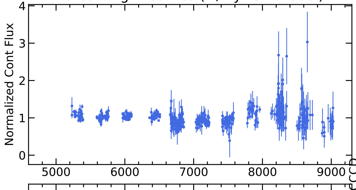
RM652 Light Curves (w/ PyROA model)
