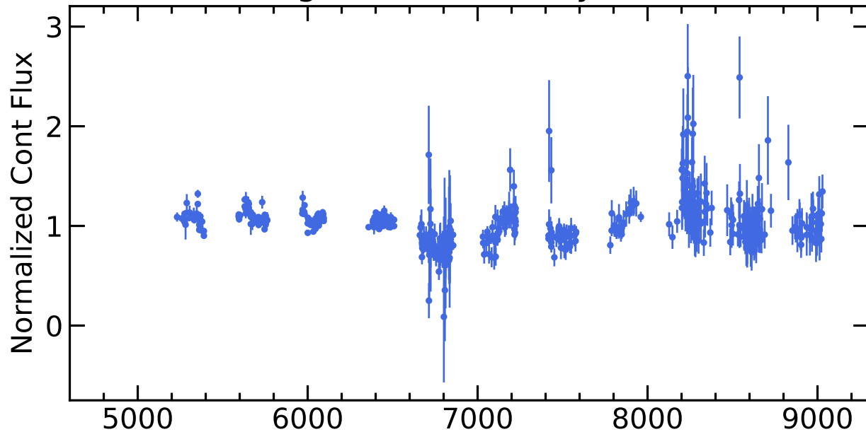
RM653 Light Curves (w/ PyROA model)
