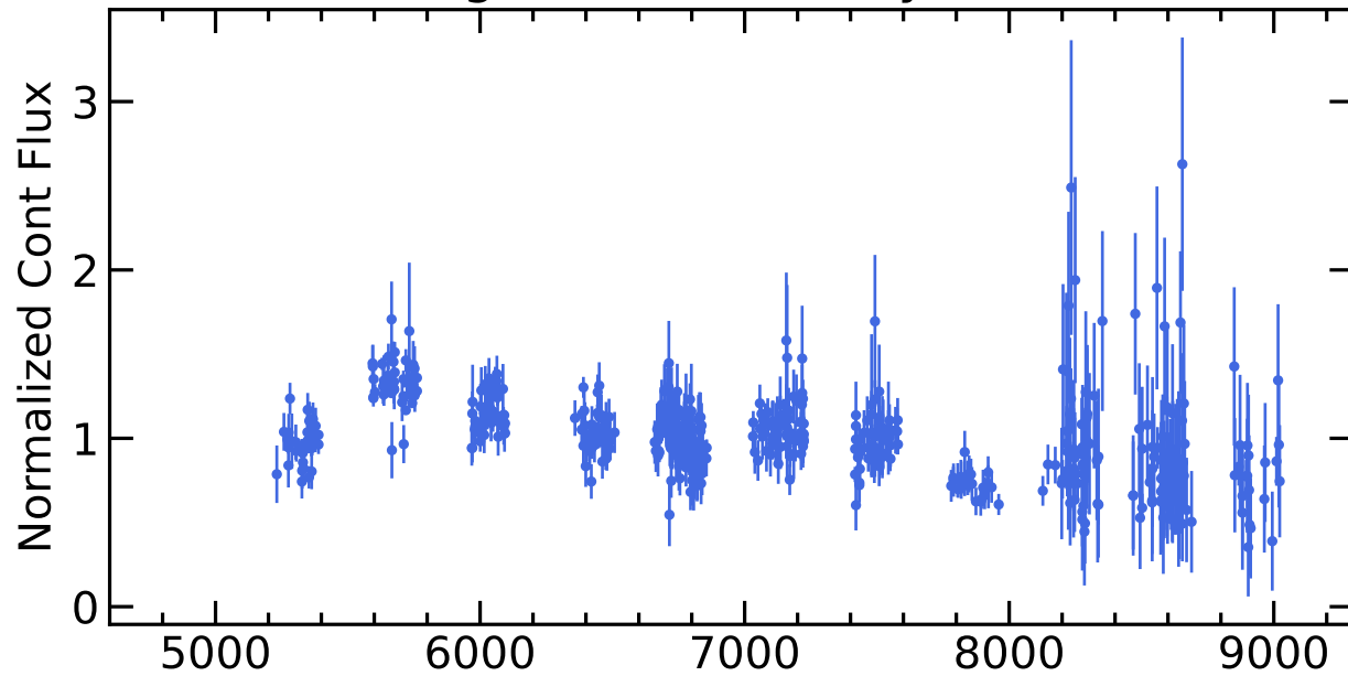
RM654 Light Curves (w/ PyROA model)
