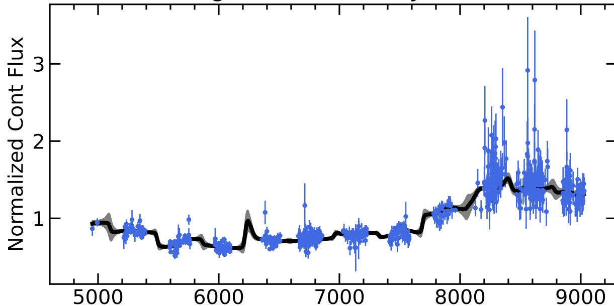
RM655 Light Curves (w/ PyROA model)
