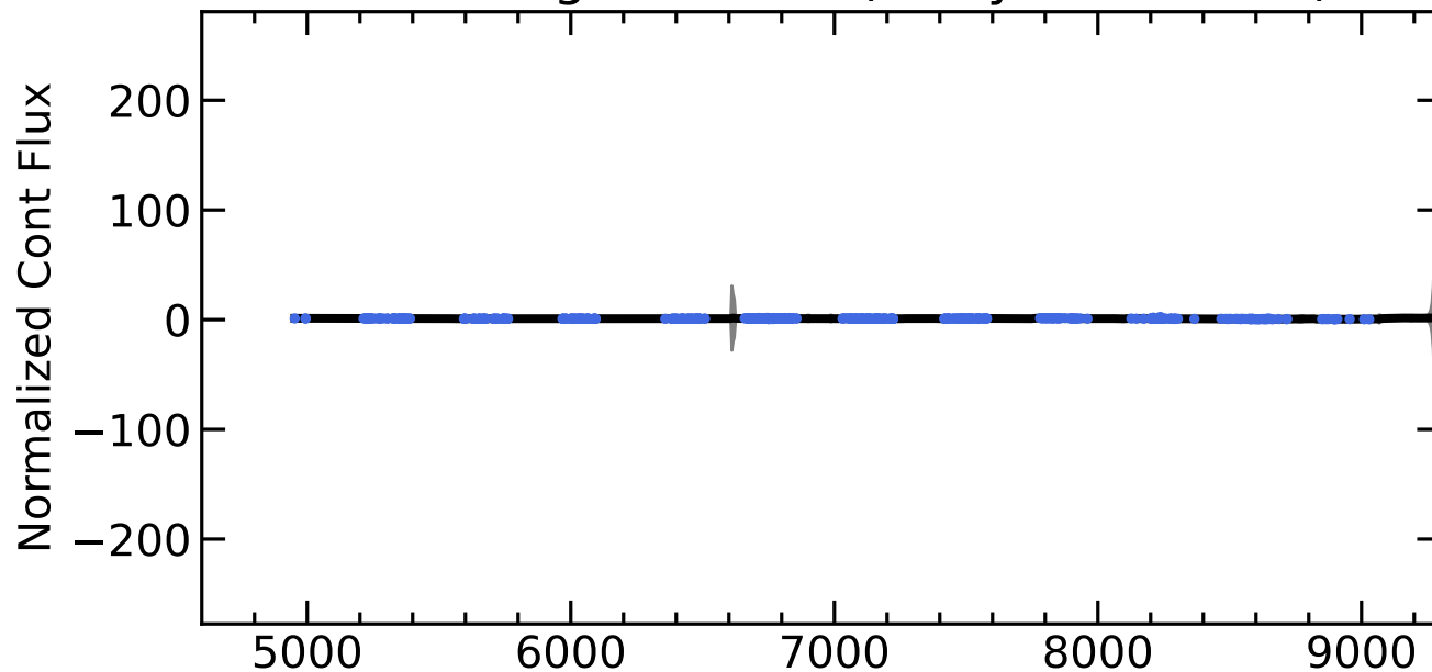
RM657 Light Curves (w/ PyROA model)
