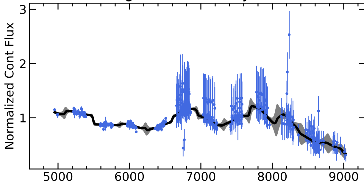
RM657 Light Curves (w/ PyROA model)
