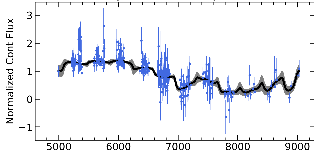
RM658 Light Curves (w/ PyROA model)
