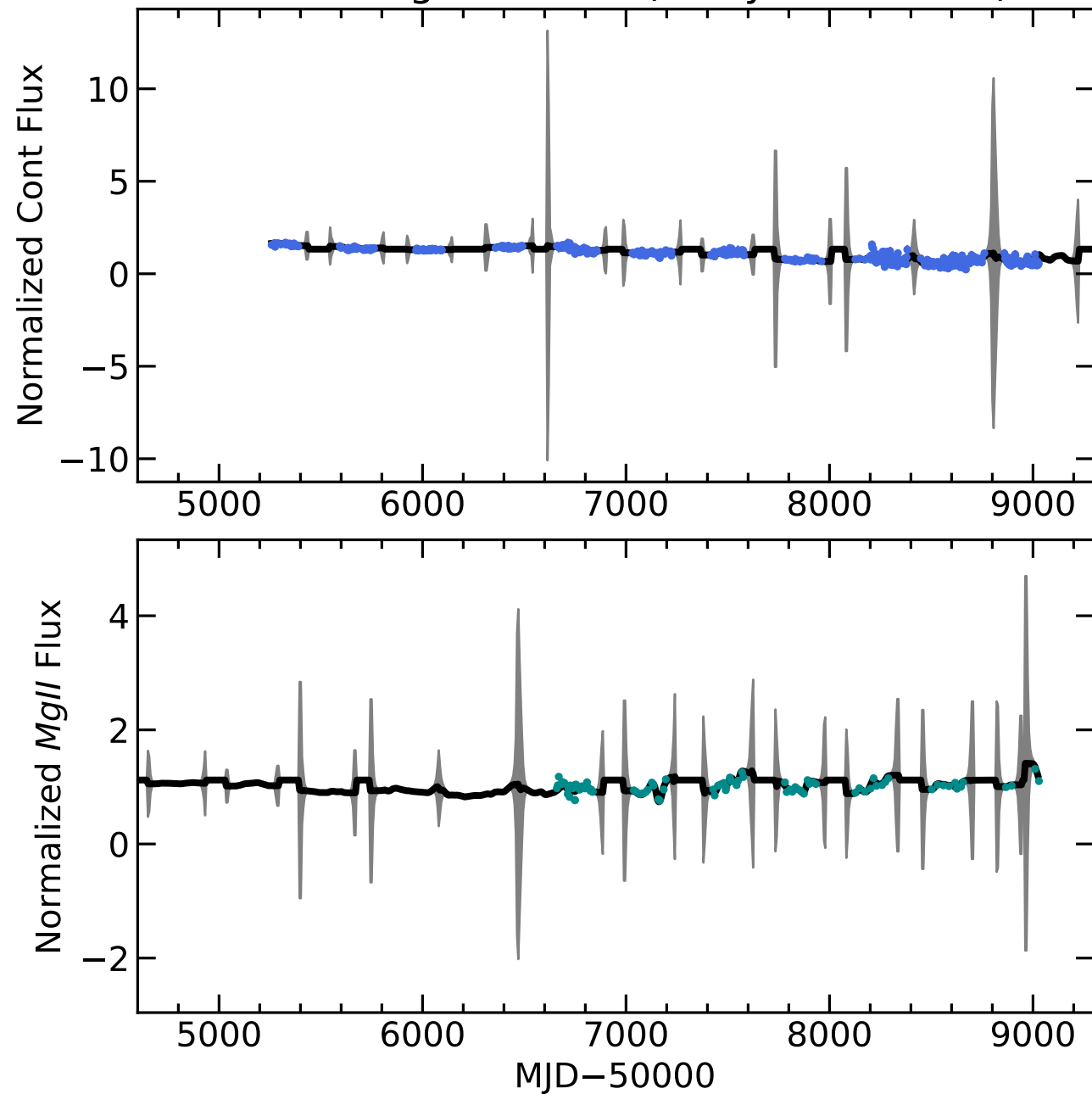
RM660 Light Curves (w/ PyROA model)
