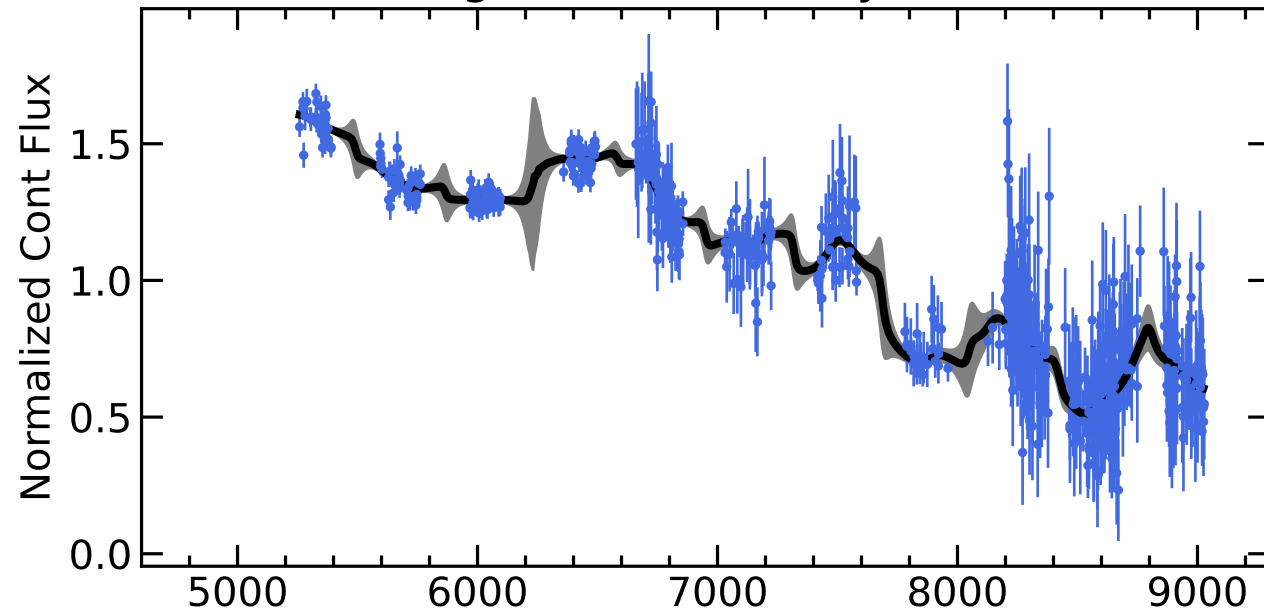
RM660 Light Curves (w/ PyROA model)
